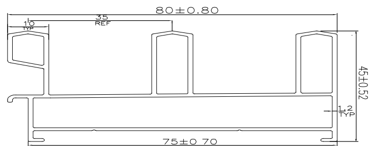
NEW STYLE 3 TRACK = 16' - 6.000 KGS
