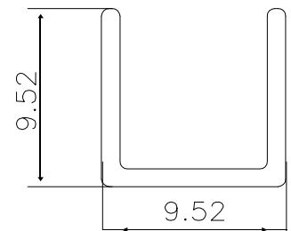
3/8 U CHANNEL = 0.068 Kg/m
