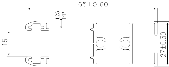
SCREW SHUTTER = 16' - 4.300 KGS
