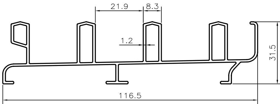
4 TRACK = 16' - 5.900 KGS
