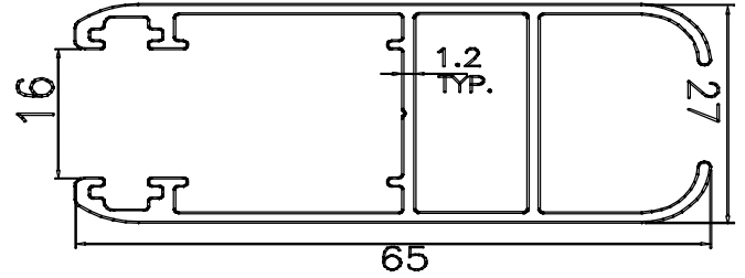
SINGLE GLASS SHUTTER = 16' - 3.500 KGS
