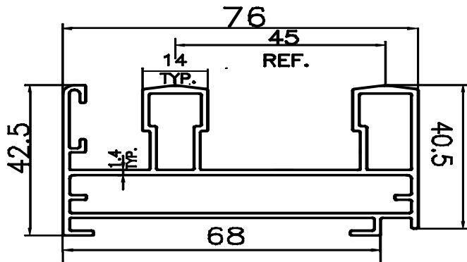
2 TRACK = 16' - 7.200 KGS
