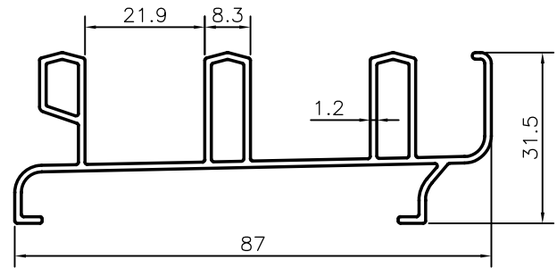
3 TRACK = 16' - 4.300 KGS
