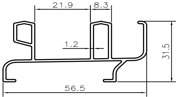
2 TRACK = 16' - 3.000 KGS
