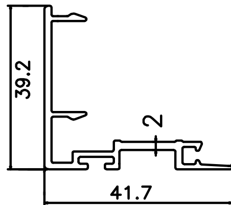
INTER LOCK = 16' - 2.200 KGS
