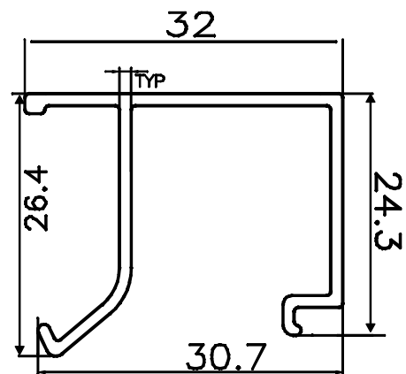
SINGLE GLASS CLIP = 16' - 1.500 KGS
