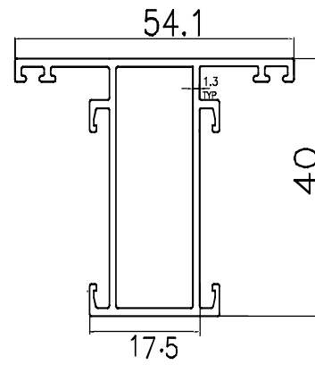
SHUTTER / MULLION = 16' - 3.300 KGS
