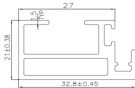
SLIM INTERLOCK = 16' - 2.750 KGS
