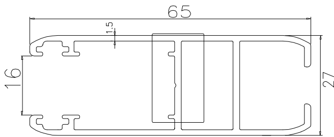
SINGLE GLASS SHUTTER HEAVY = 16' - 4.200 KGS
