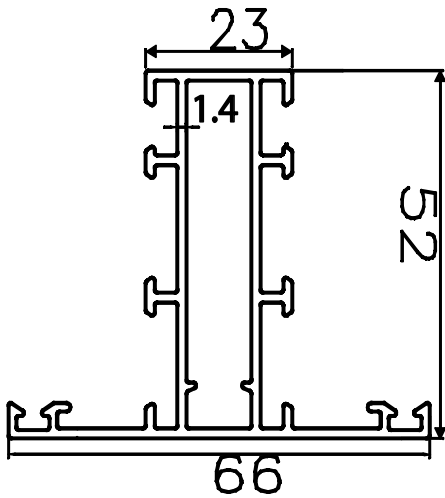
MULLION = 16' - 4.900 KGS
