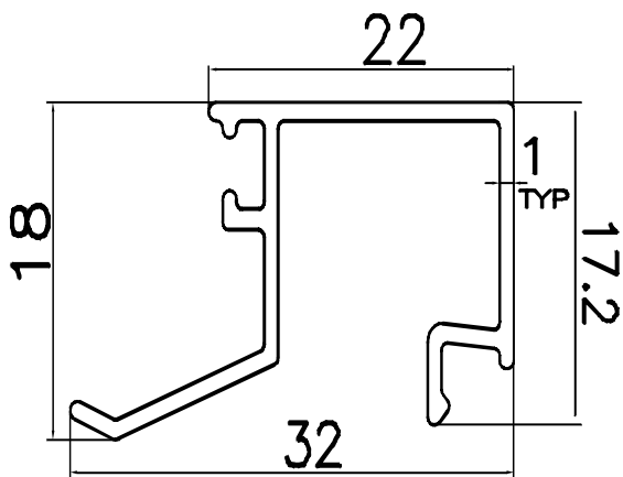
SINGLE GLASS CLIP = 16' - 1.050 KGS
